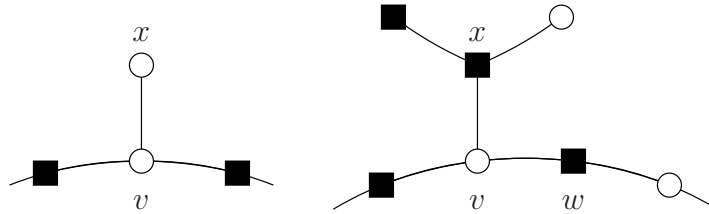
Figure 1: Examples of a flippable vertex ( v , left) and of a switchable pair of vertices ( v and w , right).
