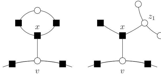
Figure 2: Two situations where v and x are not exchangeable. On the left, v and x are not exchangeable because x is the crucial vertex of an almost alternating cycle. On the right, v and x are not exchangeable because all of z_1 's neighbours (aside from x ) have the same colour as z_1 .
